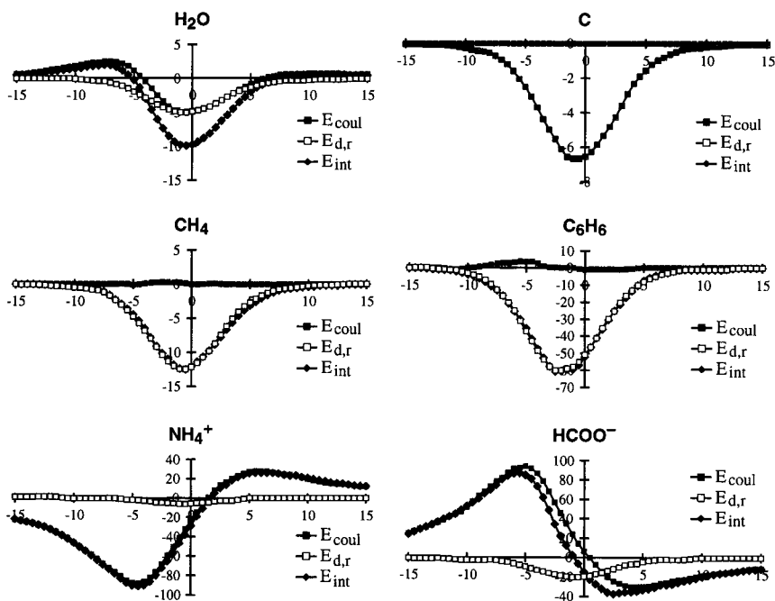
Fig. 1: Interaction energy (in \text{kJ}\cdot\text{mol}^{-1} ) profiles of simple probes entering the \beta CD cavity along the symmetry axis perpendicular to the ring plane (coordinate on the x-axis with the origin placed in the cavity center is in Å).
