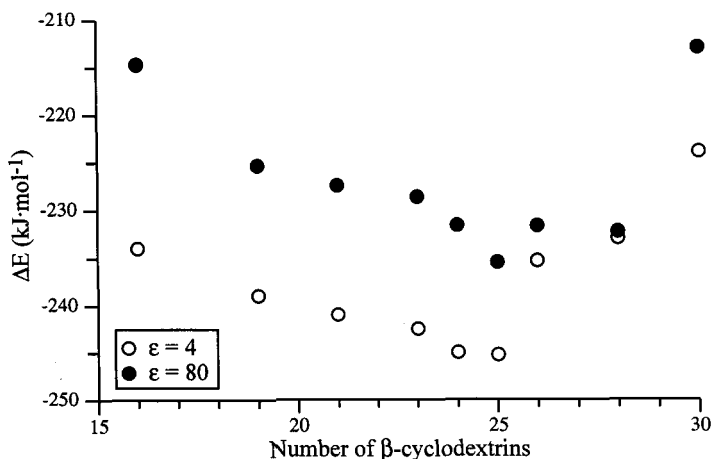
Fig. 2: Variation of the complexation energy of the system n \beta CD/IFN \alpha with number n of \beta CD molecules, in a continuum with dielectric constant 4 and 80.
